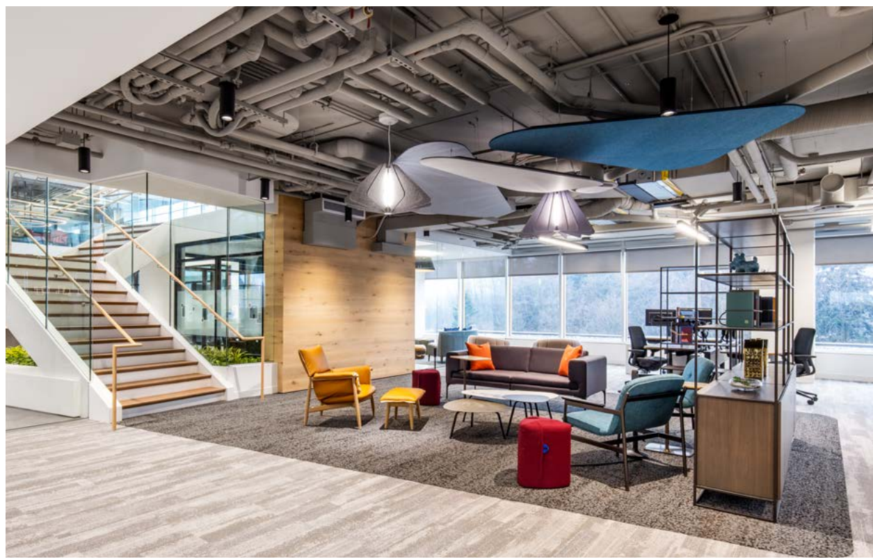
KWYET™ AVAILABLE IN STANDARD WHITE, TUNABLE WHITE, OR RGBW / COMBINATION OF TUBE LUMINAIRE & SOUND ABSORBING 9MM ACOUSTIC FINS IN 25 AVAILABLE COLORS / 80+ & 90+ CRI (R9-50) / 36" DIAMETER WITH CONE, ANGLE, OR ELLIPSE SHAPE / OPTIONAL PERFORMANCE DOWNLIGHT / EXTRUDED ACRYLIC DIFFUSER / DIE-CAST ALUMINUM END CAPS / CUSTOM SIZES, SHAPES, CLUSTERS, & CONFIGURATIONS POSSIBLE / ROHS COMPLIANT
