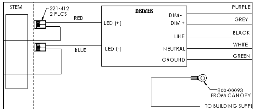
FIG. 12 – WIRE DIAGRAM
