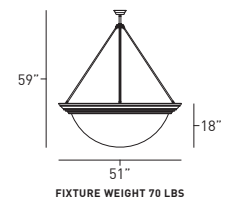
FIXTURE WEIGHT 70 LBS
