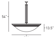
FIXTURE WEIGHT 70 LBS
