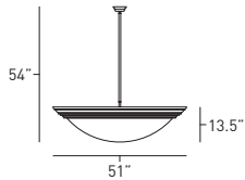
FIXTURE WEIGHT 70 LBS
