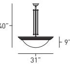
FIXTURE WEIGHT 40 LBS
