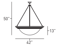
FIXTURE WEIGHT 60 LBS
